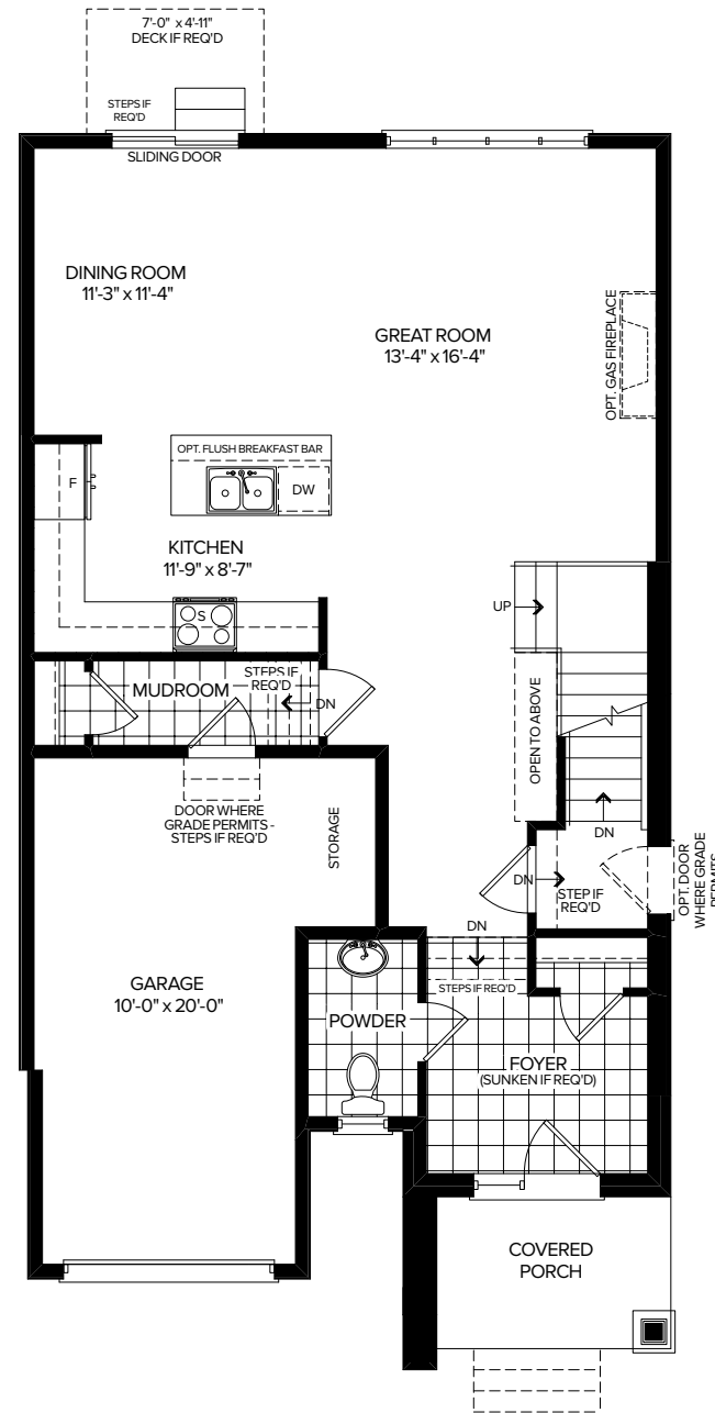
MAIN FLOOR
