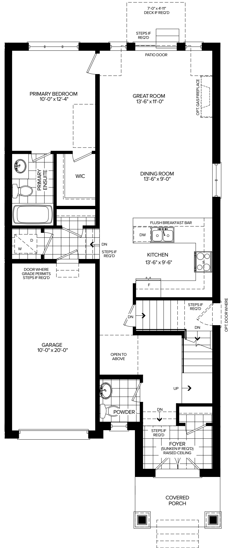
MAIN FLOOR
