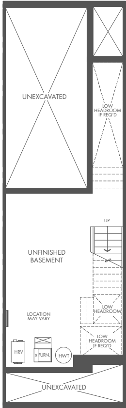
BASEMENT B
